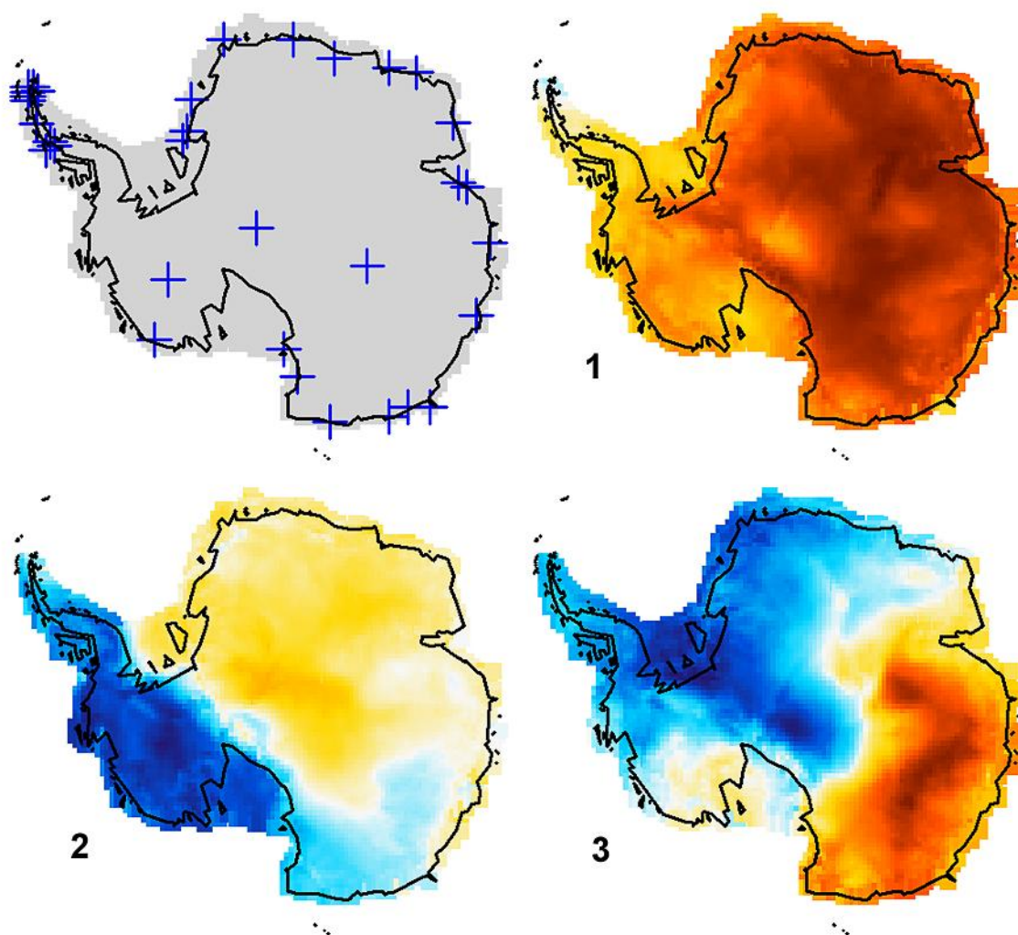
FIG. S4. Top left: on-grid S09 station locations. Other panels: AVHRR spatial eigenvectors, with eigenvector order listed.
