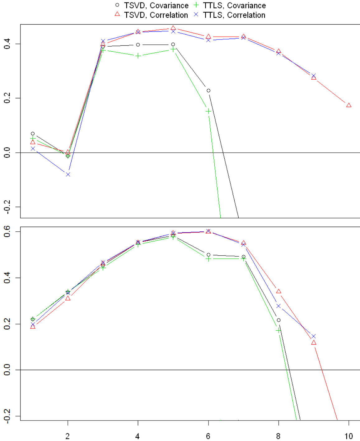
FIG. S9. Comparison of TSVD vs. TTLS algorithms for station set Grid.1C. Top panel: minimum CE from early/late withholding of verification stations. Bottom panel: CE results for random withholding of 5% of the data.
