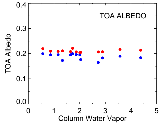
Chou Model (SSA = 1, g = 0.7)
