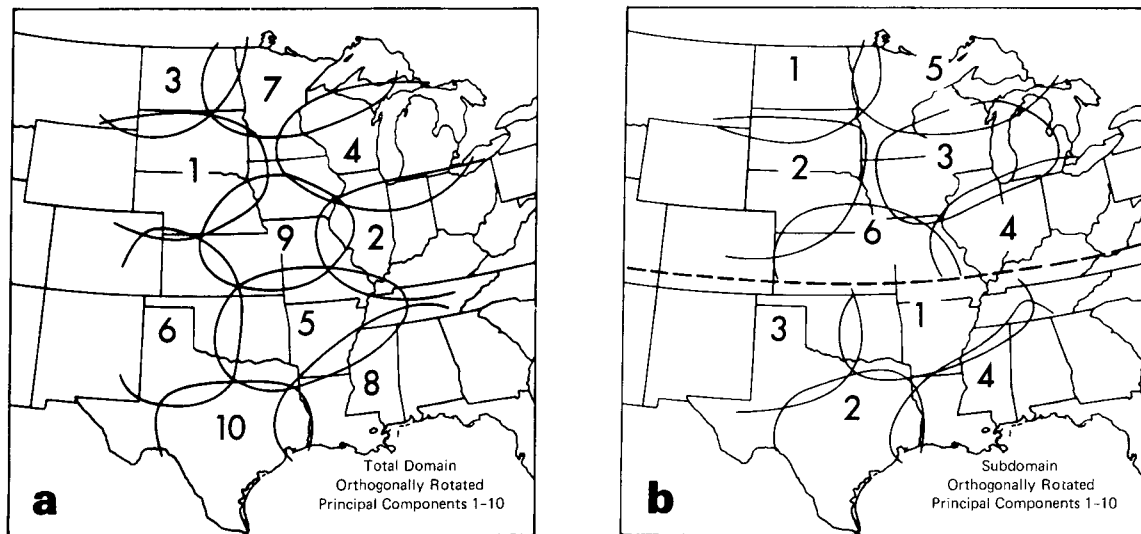
Figure 3. Regionalization of the central United States for 3-day summer rainfall totals for orthogonally rotated (Varimax criterion) principal components. The regional boundaries are the 0.4 loading isopleths for individual PCs. The results for the full domain appear in (a) and those computed separately for the northern and southern halves of the domain are shown in (b). The zonal division is given by the thick broken line. (Taken from Richman and Lamb, 1985)
