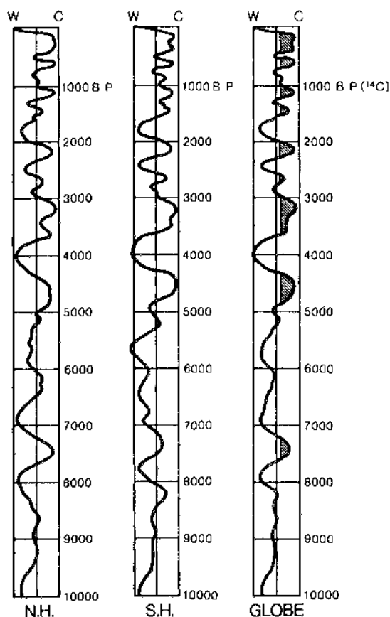
FIGURE 1. Alpine glacier advance and retreat chronologies for the Northern Hemisphere (N.H.), Southern Hemisphere (S.H.) and globe based on Röthlisberger (1986). W and C refer to warm (glaciers less advanced) and cold (glaciers more advanced).
