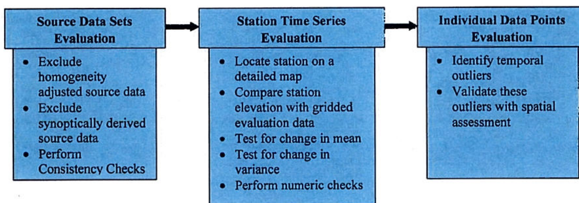
Figure 2. Flow chart of NOAA quality control tests for data incorporated into GHCN-M Version 2
